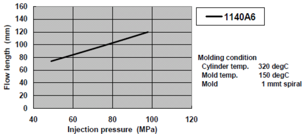
Figure 3-1 Flowability (1 mmt)
