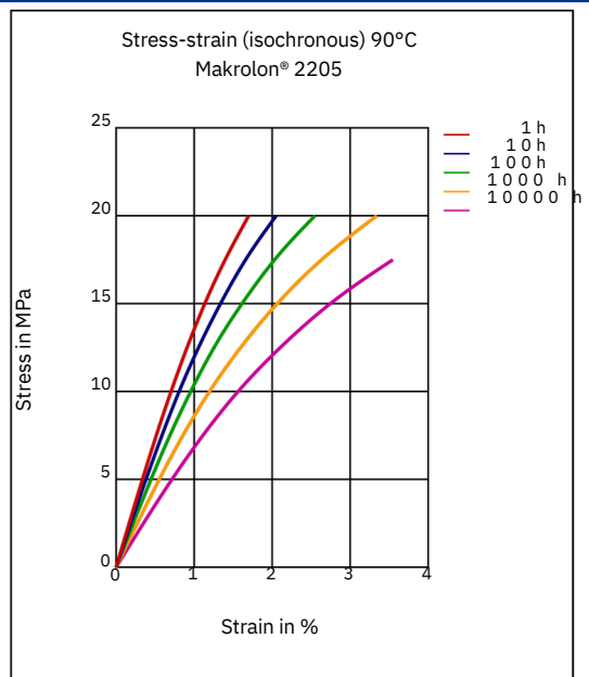
Stress-strain (isochronous) 90°C
