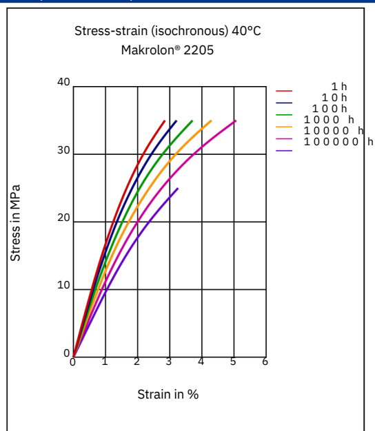
Stress-strain (isochronous) 40°C
